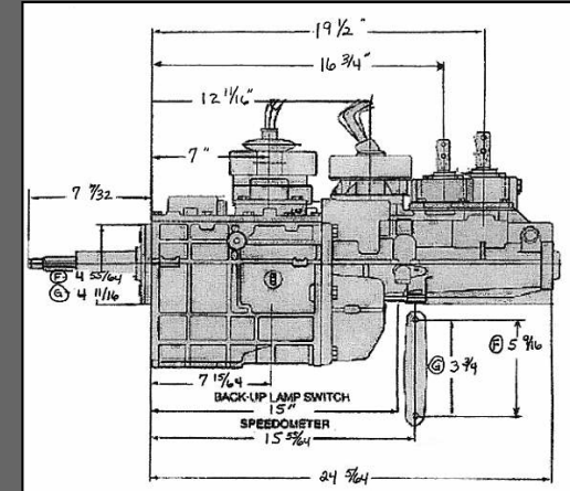
Tremec TKO 500 & 600
